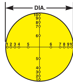
Log-linear traverse for round ducts, two-diameter approach.
