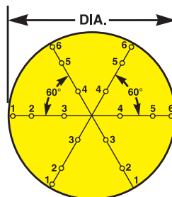
Log linear-traverse for round ducts, three-diameter approach.
