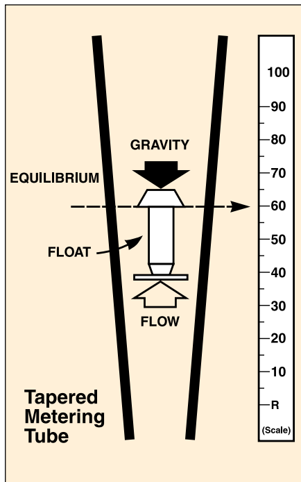
Variable area flow meter, also called a rotameter, has a float that moves up or down in a tapered tube. The distance it moves is proportional to the liquid flowrate and the annular area between the float and the tube well.
