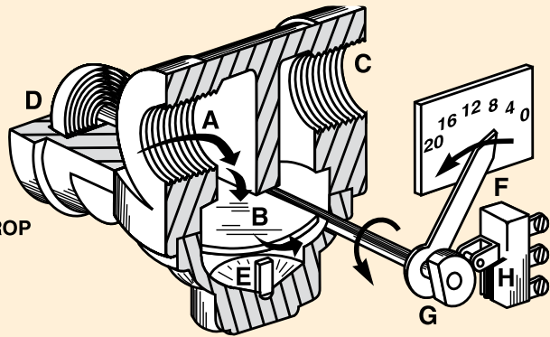
Flowmeters Operating Principle of FL-X Series
