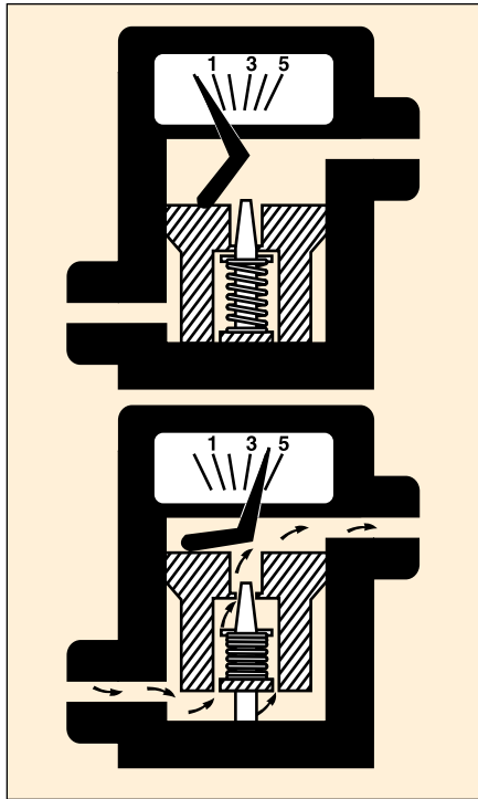
Flowmeters Operating Principle of FL-O Series
