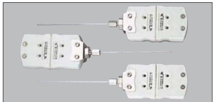
For Fast Response, RTD Probes Can Be Constructed with 1/8" Diameter Sheaths (Miniature Connectors Available)
