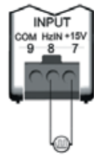
NAMUR or PNP Sensor Powered from the DRF-FR Signal Conditioner
