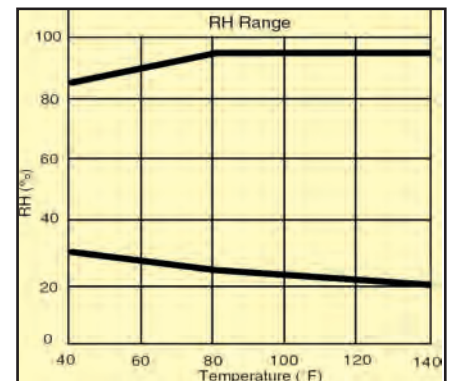
Relative Humidity Measurement Range vs. Temperature
