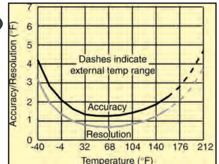
Temperature Measurement Accuracy/Resolution
