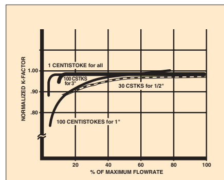
Figure 4: Viscosity effect on a turbine meter
