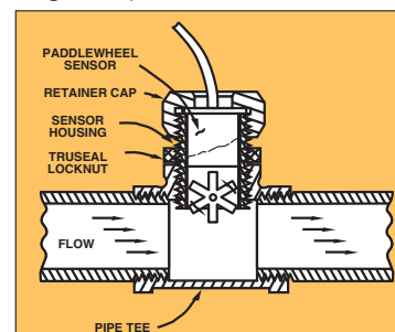
Figure 7: Paddlewheel flow sensor installation and operation
