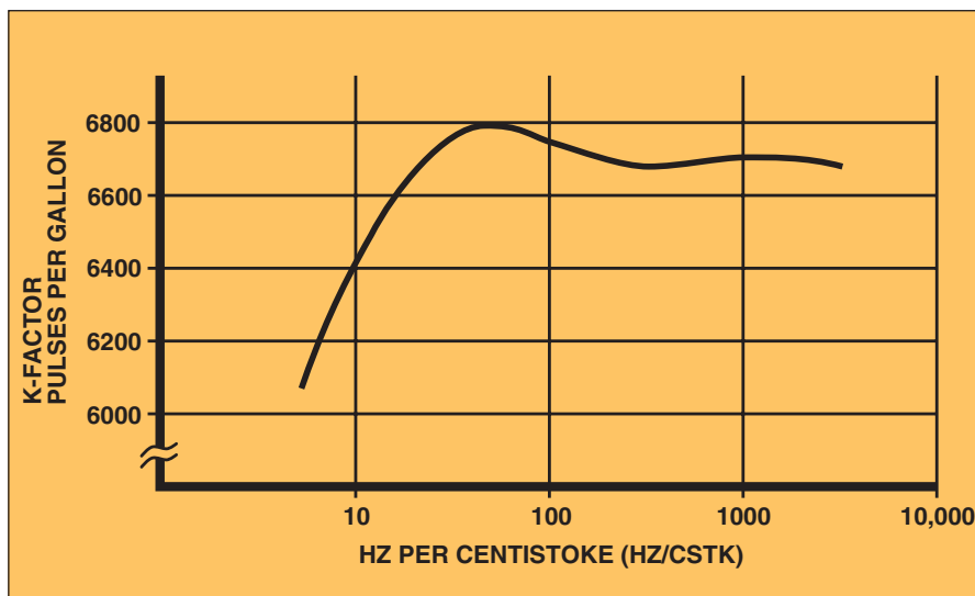
Figure 1: Universal viscosity curve
